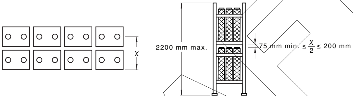
Figure C.3 — Clearances for other types (front view)
