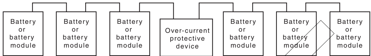
Figure 6.15 — Overcurrent protection device in series in middle of battery string or battery modules
