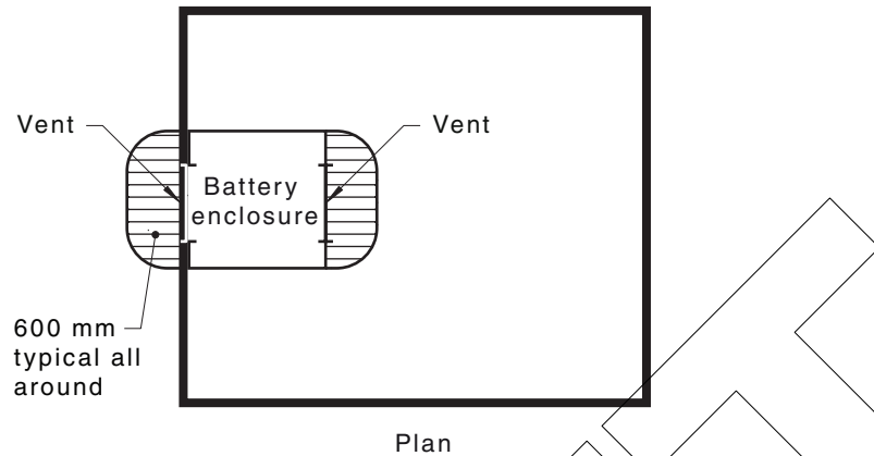
Figure 6.17 — Battery system enclosure within a room where the battery system enclosure is vented to outside the building
