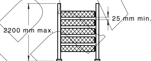
Figure C.4 — Single-row, single-tier battery stand
