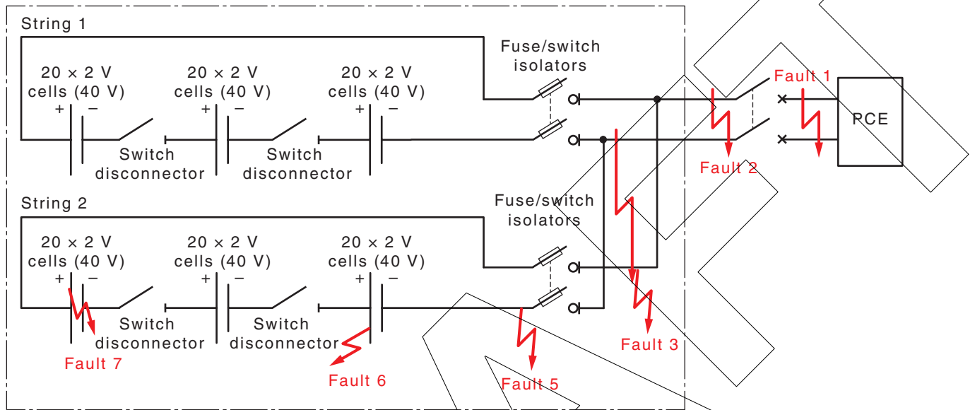
Figure G.2 — Example: Typical configuration and possible d.c. arc fault scenarios
