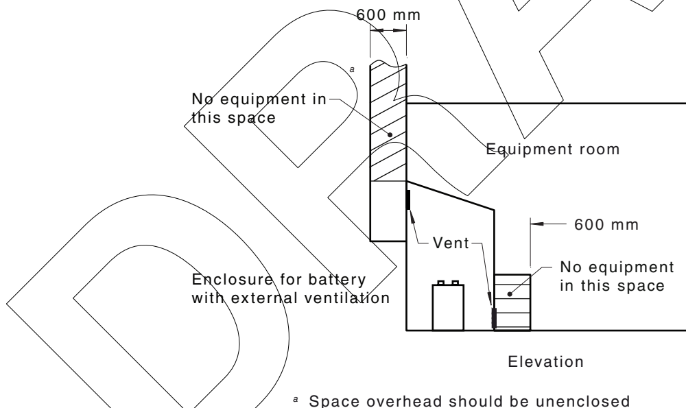
Figure 6.16 — Battery system enclosure within a room where the battery system enclosure is vented to outside the building
