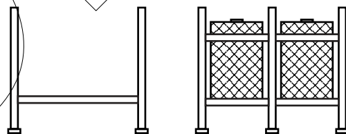
Figure C.5 — Double-row, single-tier battery stand
