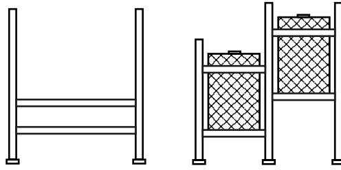
Figure C.6 — Double row, single tier stepped battery stand
