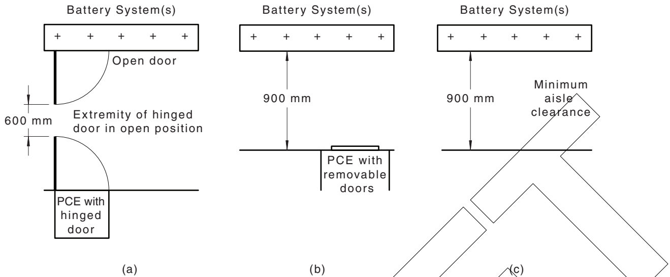
Figure 6.3 — Minimum aisle width requirements for systems greater than DVC-A
