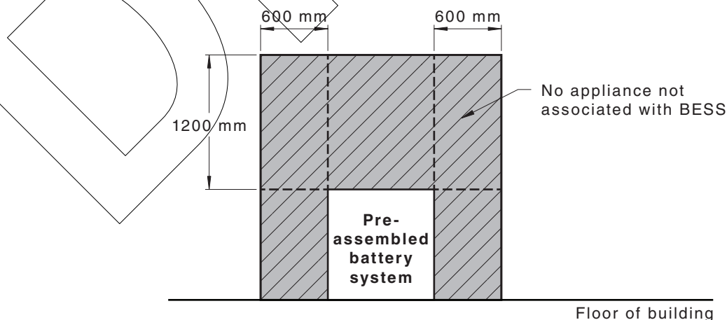
Figure 5.1 — Restricted zones for equipment not associated with the Battery systems
