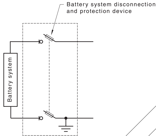
Figure 5.7 — Location of earth connection on single battery system
