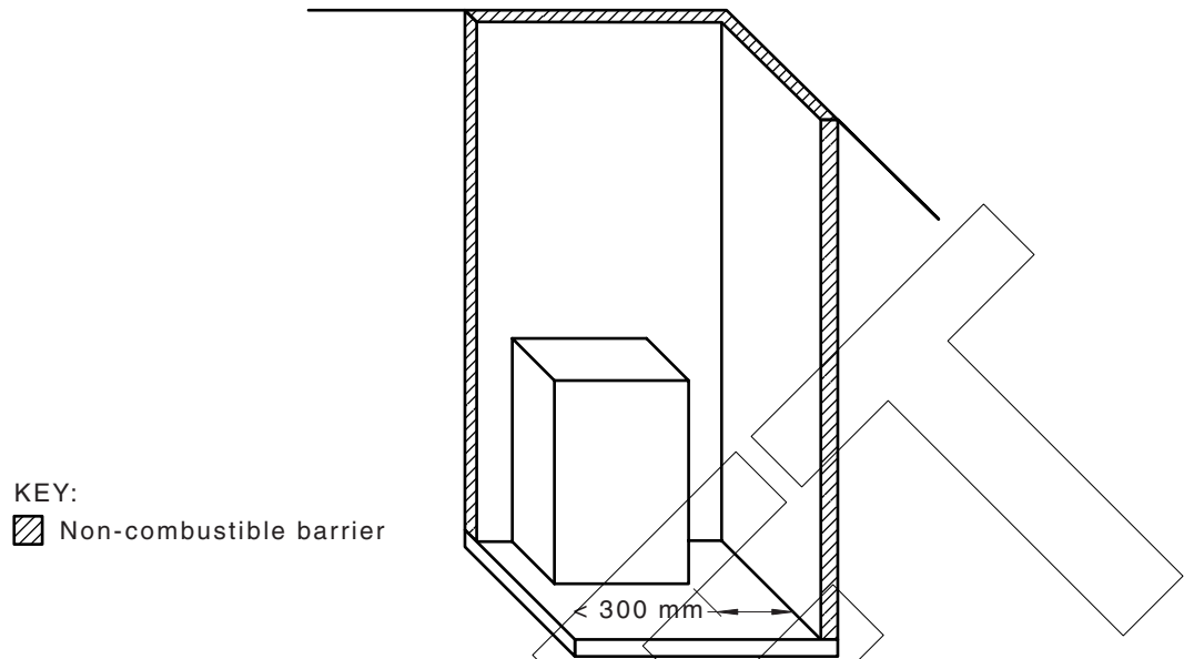
Figure E.4 — Battery system or BESS installed in the corner
