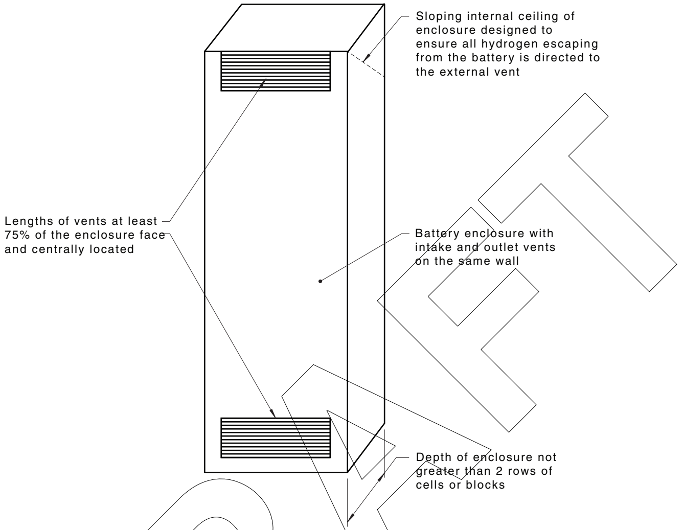
Figure D.4 — Example battery system enclosure with the intake and outlet vents on the same wall
