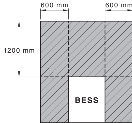
Figure 4.2 — Barrier zones for pre-assembled integrated BESS installed on or near a habitable room facing wall
