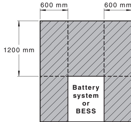
Figure 6.2 — Barrier zones for battery systems or BESS installed on or near a habitable room facing wall
