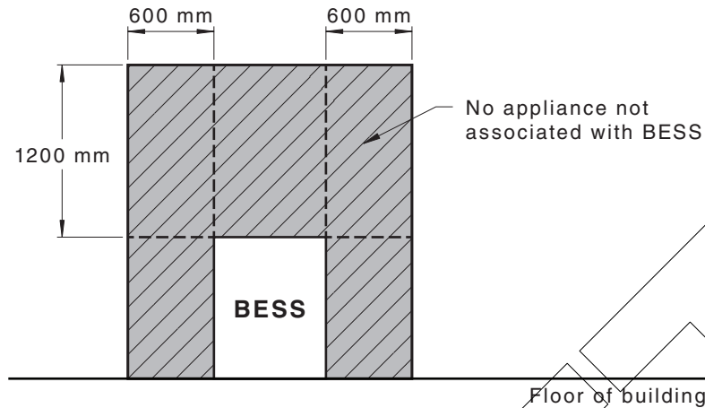
Figure 4.1 — Restricted zones for equipment not associated with the BESS
