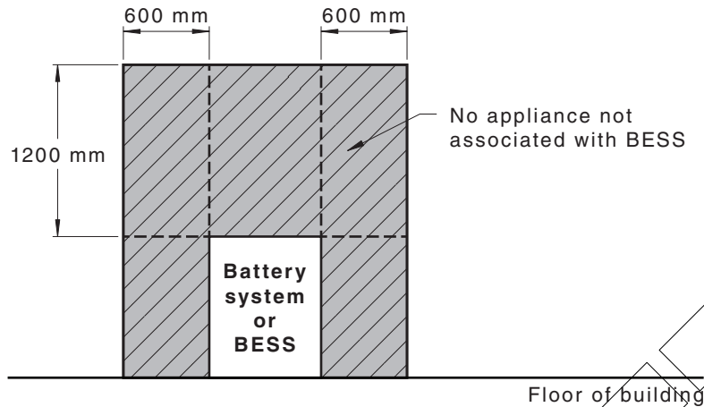
Figure 6.1 — Restricted zones for appliances not associated with the battery systems
